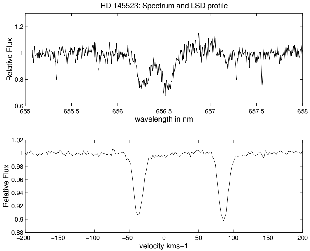
Figure 1: The top plot represents a small section of the spectrum taken at Mt Stromlo Observatory of HD 145523. The bottom plot is the LSD profile for this binary star. More than 600 individual photospheric line features have been combined to increase the S/N ratio.
