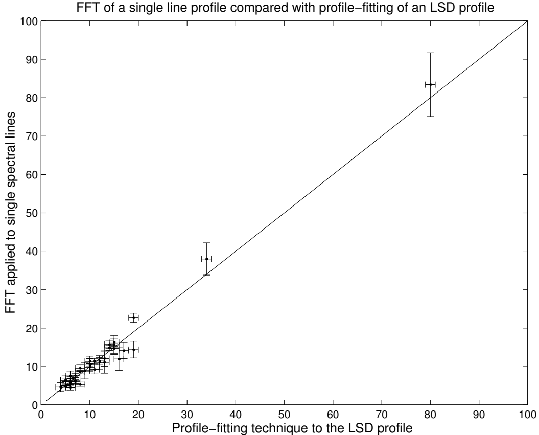
Figure 2: The relationship between the results of v \sin i measurements found using an FFT of a single line profile compared with v \sin i measurements found using profile fitting of the LSD profile using a rotationally broadened spectrum from a standard star of similar spectral type.
