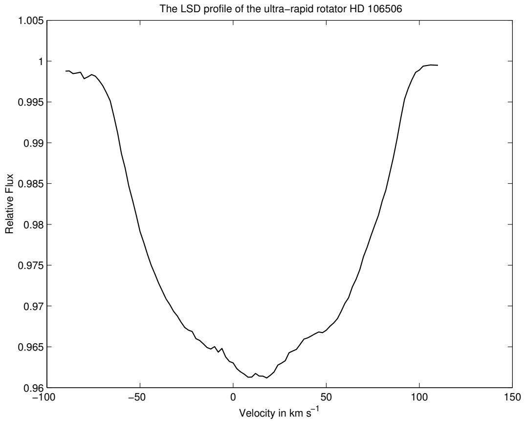
Figure 6: The LSD profile for HD 106506, an active, young, apparently single star with very rapid rotation ( v \sin i = 80 \text{ km s}^{-1} ). The distortion of the profile near zero velocity is suggestive of spot features on the stellar surface.
