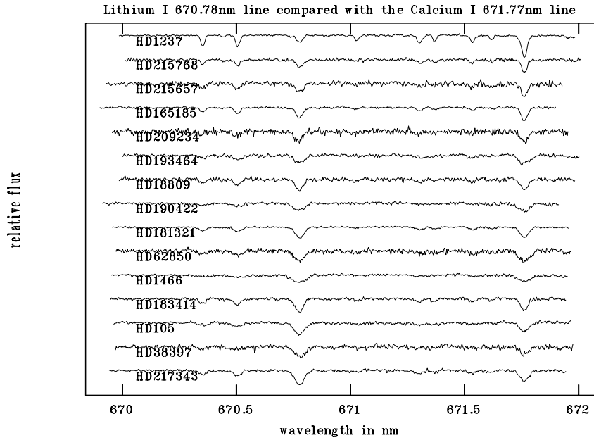
Figure 5: The spectra of 15 young stars in the sample, as judged by their strong LiI 670.78-nm line. The CaI 671.77-nm feature is shown for comparison.
