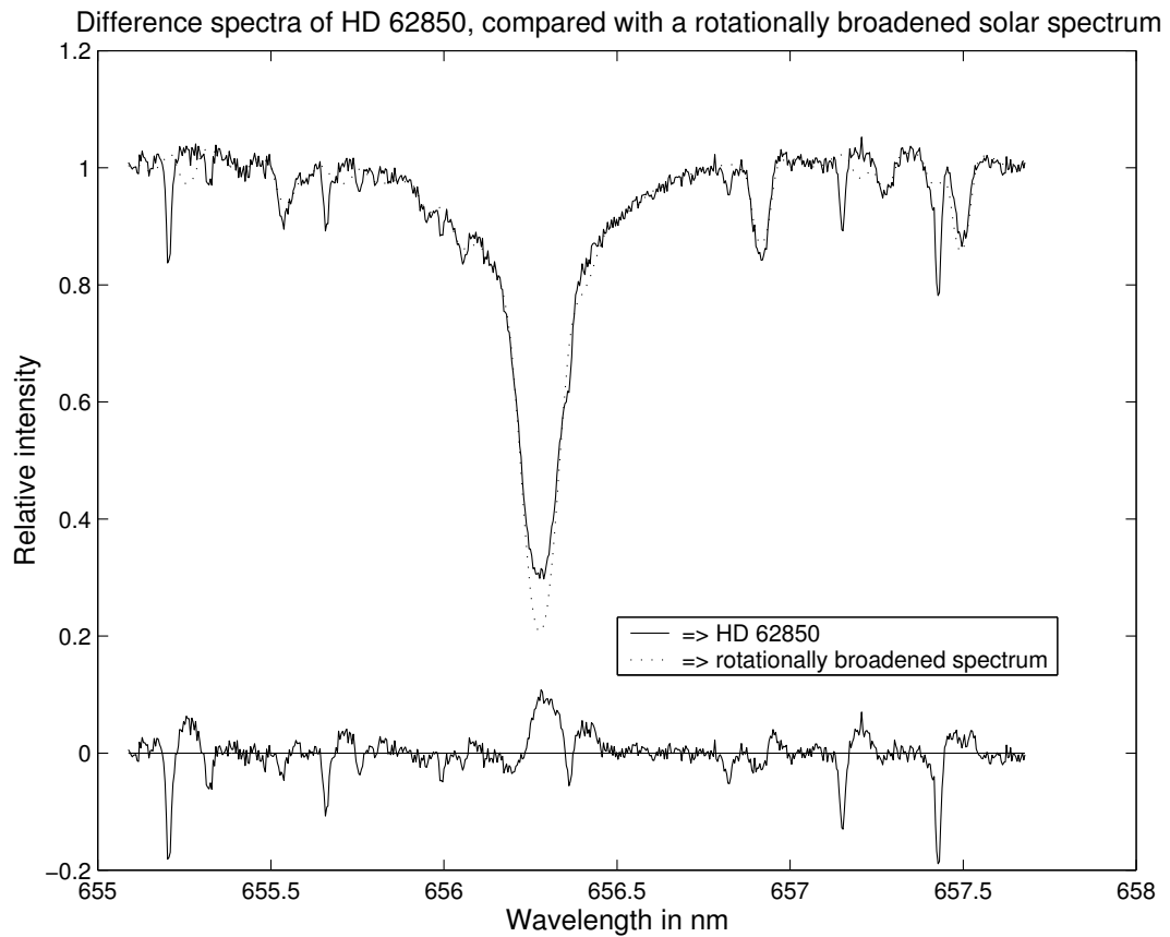
Figure 3: The H\alpha emission of HD 62850. The upper plot is a spectrum of the star prior to the subtraction of a rotationally broadened spectrum of a low-activity star (i.e. the solar spectrum). The lower plot shows the resulting net H\alpha emission for HD 62850 used to measure its EEW and demonstrating the filling-in of the photospheric line by chromospheric activity.
