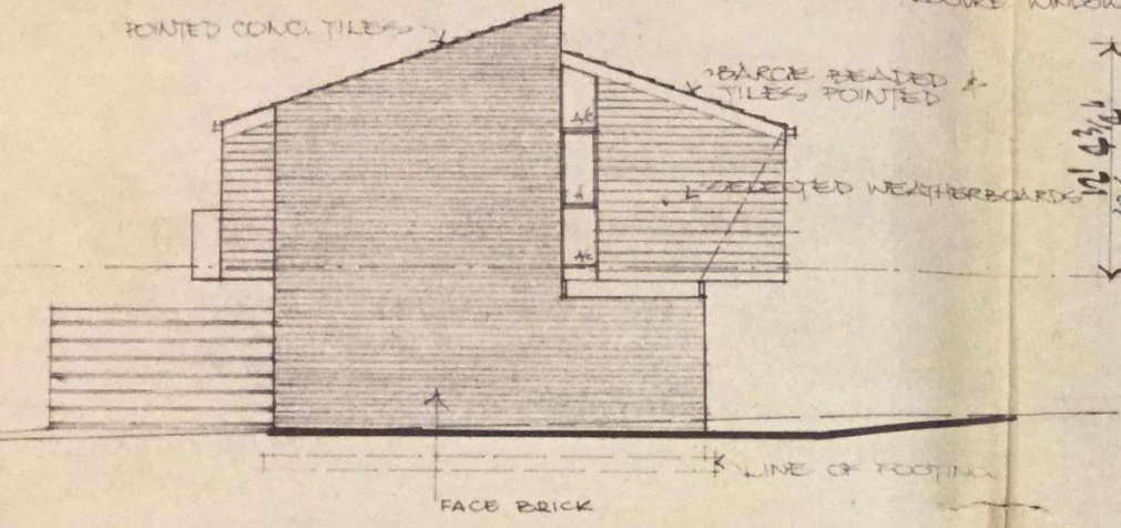
SOUTH ELEVATION.
