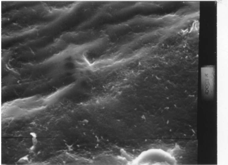
Figure 12: 1500 Times Microscopy Photo of Diffusion of Araldite into Thermoplastic Composite
