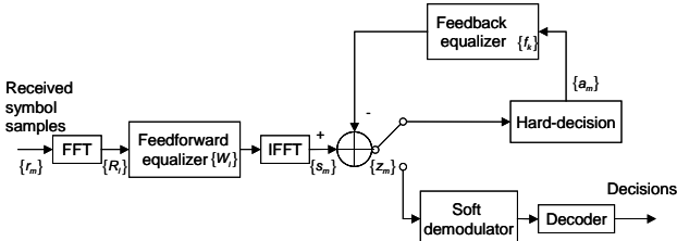
Fig.3.Iterative DFE with cyclic detection
