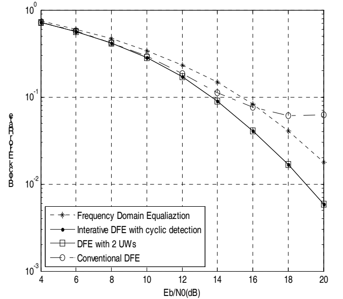
Fig.5. Performance comparison among several equalization algorithms (100 sub-carriers are occupied)
