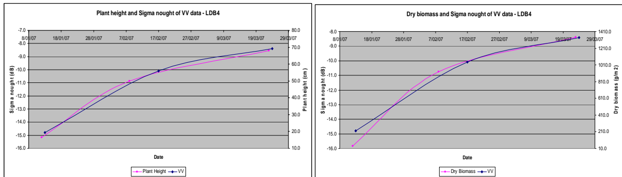
Figure 4: Temporal variation of \sigma^0 of VV and plant height (left), biomass (right)
