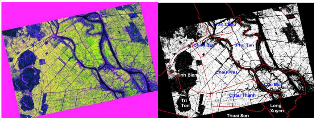
Figure 6: Colour composite (HH-HH/VV-VV) image (left) and rice/non rice image (right)
