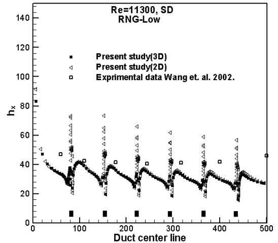
Fig. 4 Two and three dimensional total convective heat transfer coefficient along the center line of straight duct
