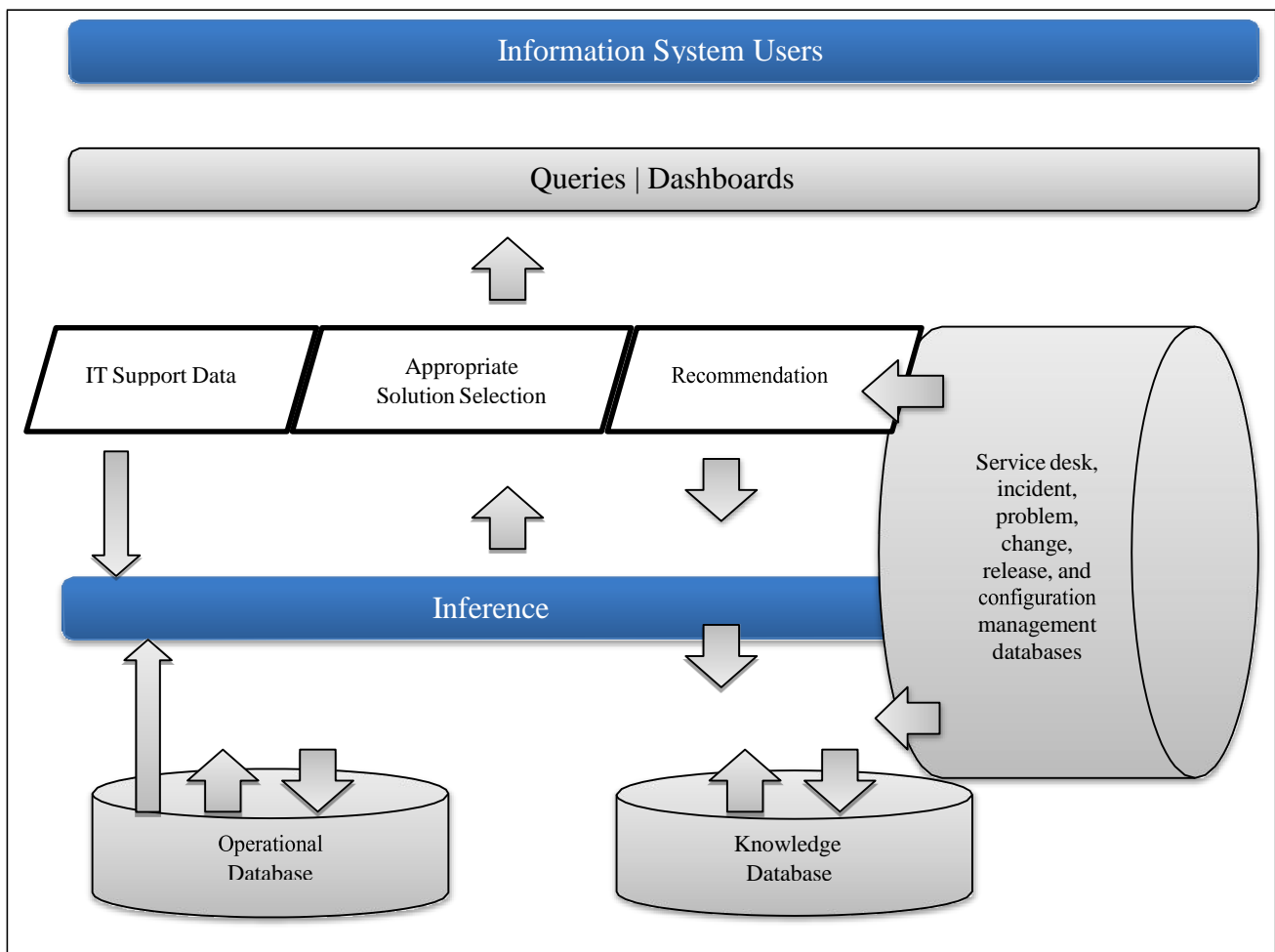
Figure 2. Architecture of a Decision Support Recommendation System
