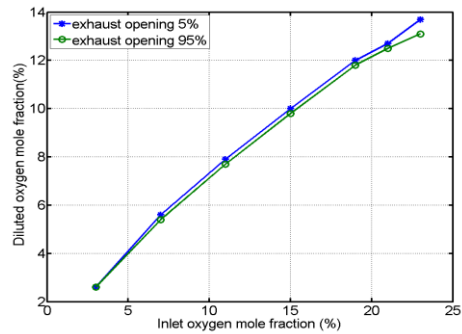
Figure 8: Oxygen mole fraction for inlet oxidant (x-axis) and diluted oxidant that entering combustion chamber (y-axis).
