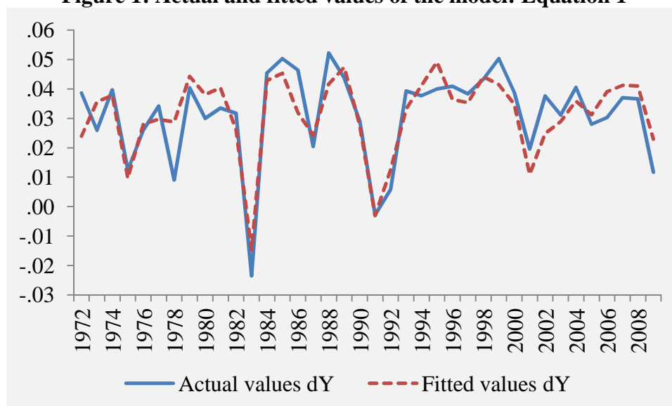
Figure 1: Actual and fitted values of the model: Equation 1
