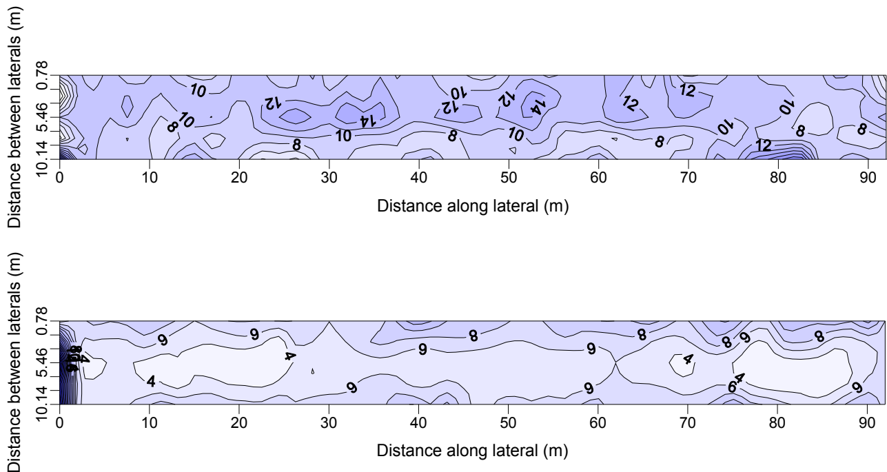
Figure 3. Whole field \Delta EC_a (a) for the 4 th (on-ground) and (b) 10 th (elevated) irrigation measurements.
