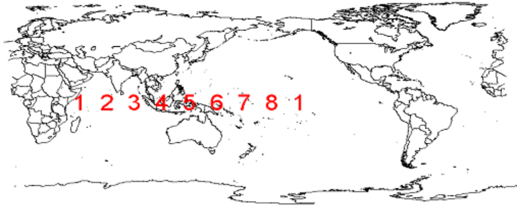
Figure 1: Approximate locations of the MJO centre of convection RMM Index phases 1-8. Phase 1 includes signals both from the initiation of an MJO event in the western Indian Ocean basin and the breakdown of MJO events in the mid-Pacific Ocean. During phases 2 through 8 the MJO travels east at 4-10 days/phase.
