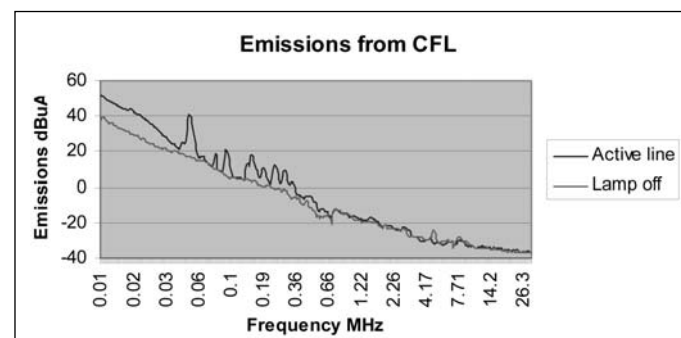
Figure 11. Conducted emissions on the active line of a compact fluorescent lamp. The upper trace is emissions on the active line and the lower trace is the measurement with the lamp turned off.
