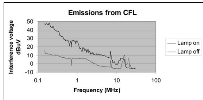
Figure 10. Conducted emissions from a typical compact fluorescent lamp. The upper trace is emissions on active and neutral lines which are virtually identical and the lower trace is the measurement with the lamp turned off.
