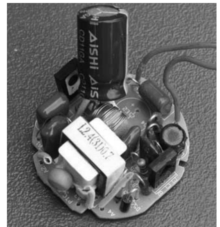
Figure 6. The ballast circuit of the compact fluorescent lamp.
