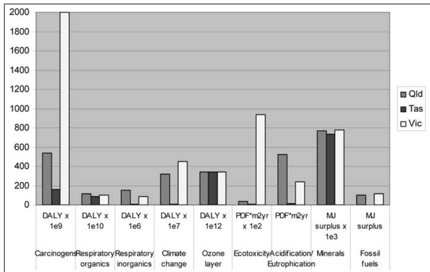
Figure 7. Comparison of environmental impact of a compact fluorescent lamp using three different sources of energy: Queensland – Black coal, Tasmania – Hydroelectricity, Victoria – Brown coal.
