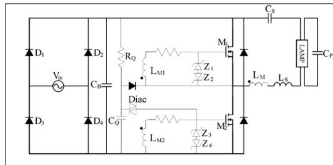
Figure 9. Probable topology of ballast circuit of CFL studied. Source: Dalla Costa et al. (2001) figure 1 (b).
